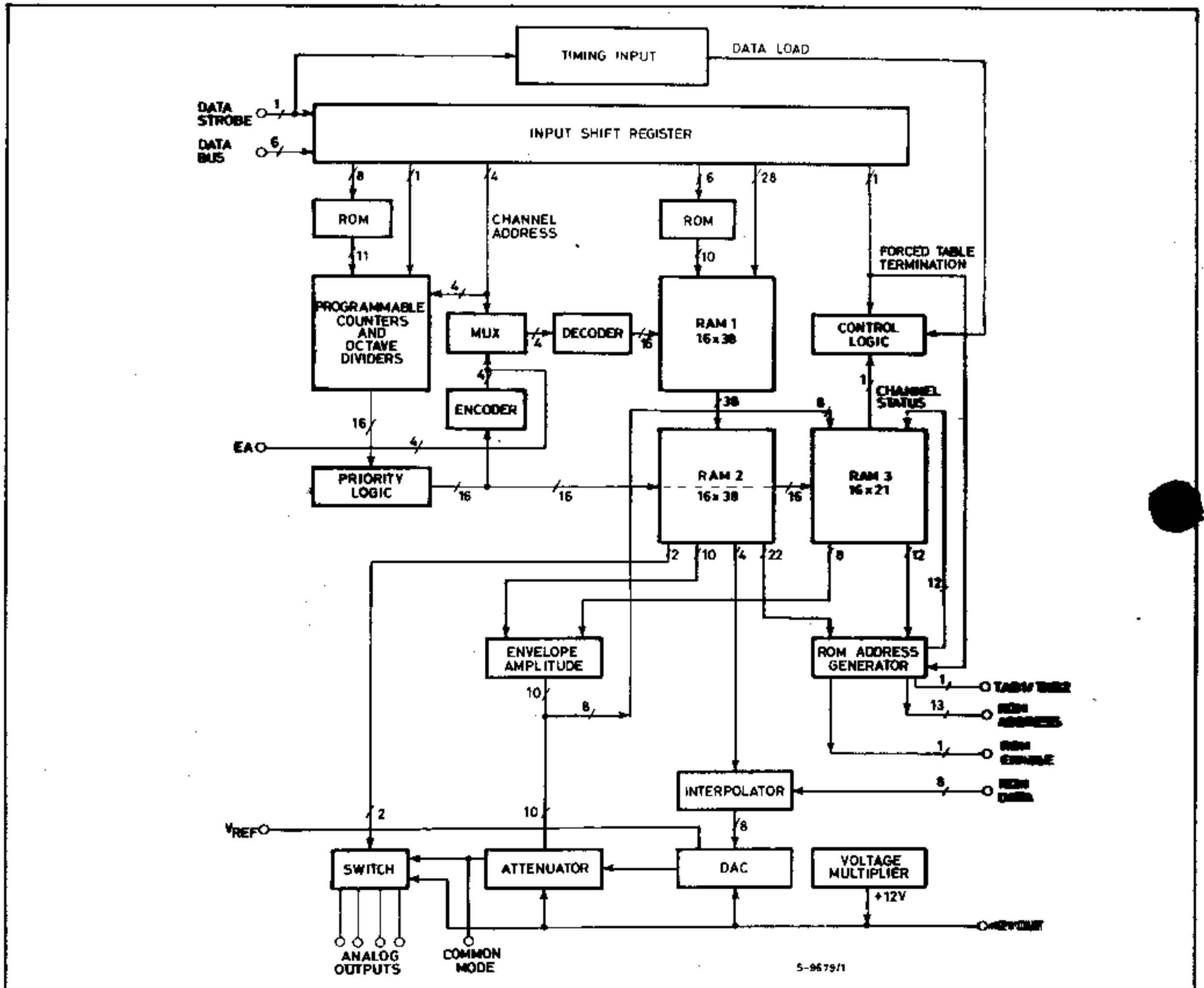
Fig. 1 - Block Diagram
